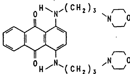
Compound 1c
